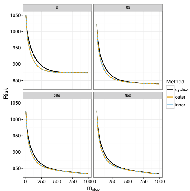
Fig. 2 Convergence speed (regarding the number of boosting iterations m ) with 6 informative and p_{n-\text{inf}} = 0, 50, 250 and 500 additional noise variables
