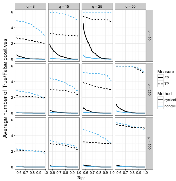
Fig. 5 Unbalanced case with normal distribution (Scenario 1B)
